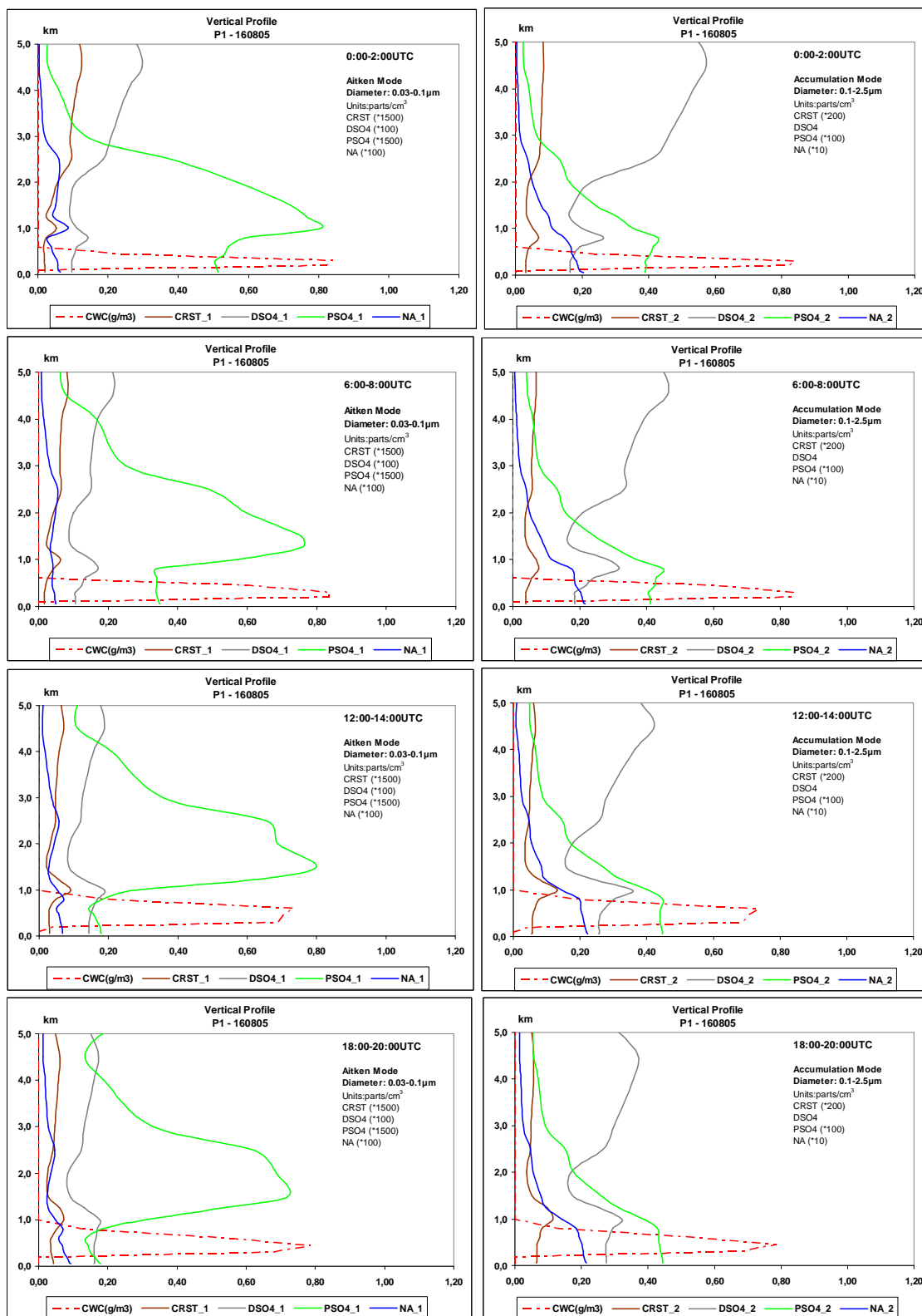
Fig. 9. Vertical profile of the condensed cloud water content CWC ( \text{g/m}^3 ) and the aerosol number concentration (particles/ \text{cm}^3 ) at location P1 (lat, lon)=(23.5° N, 18.5° W). The left panels show the aerosols in the size section 1: 0.03–0.1 \mu\text{m} . The right panels show the aerosols in the size section 2: 0.1–2.5 \mu\text{m} . Day: 16 August 2005.
